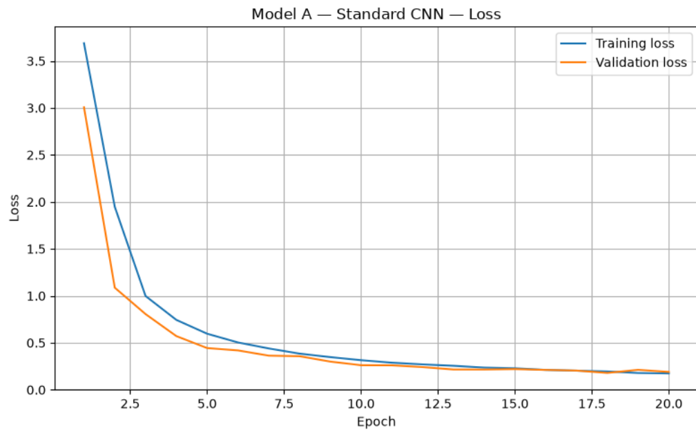
Figure 2.2: Losses of Training and validation curves for Model A.
