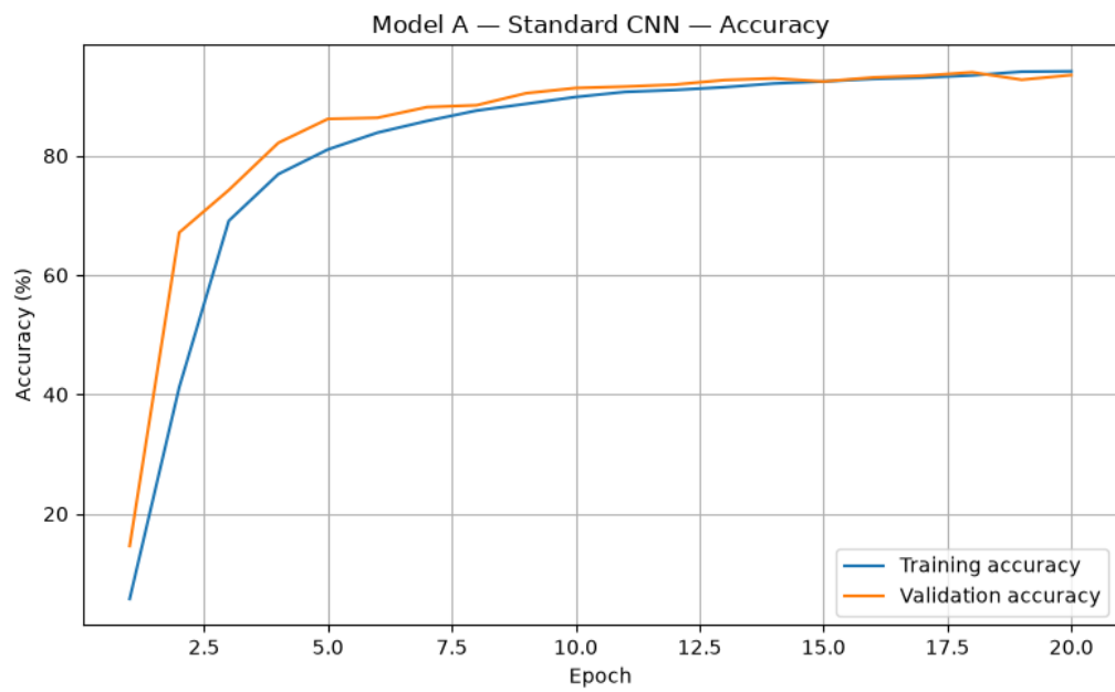
Figure 2.3: Accuracy Training and validation curves for Model A.
